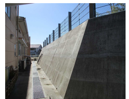
[重力式擁壁]
